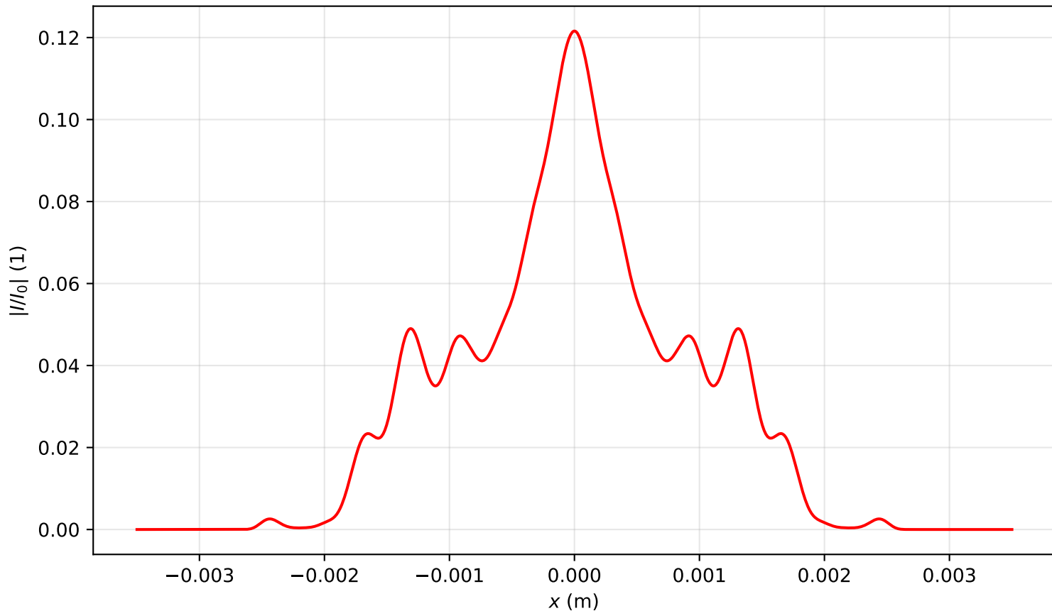
Intensity profile I(x, y = 0, z = 3.344)/I_0 , P_{in}=5.5P_{cr} , artificial time
